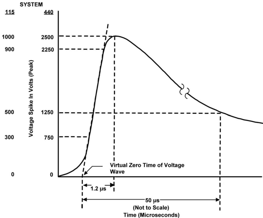
FIGURE 5. Voltage spike.
