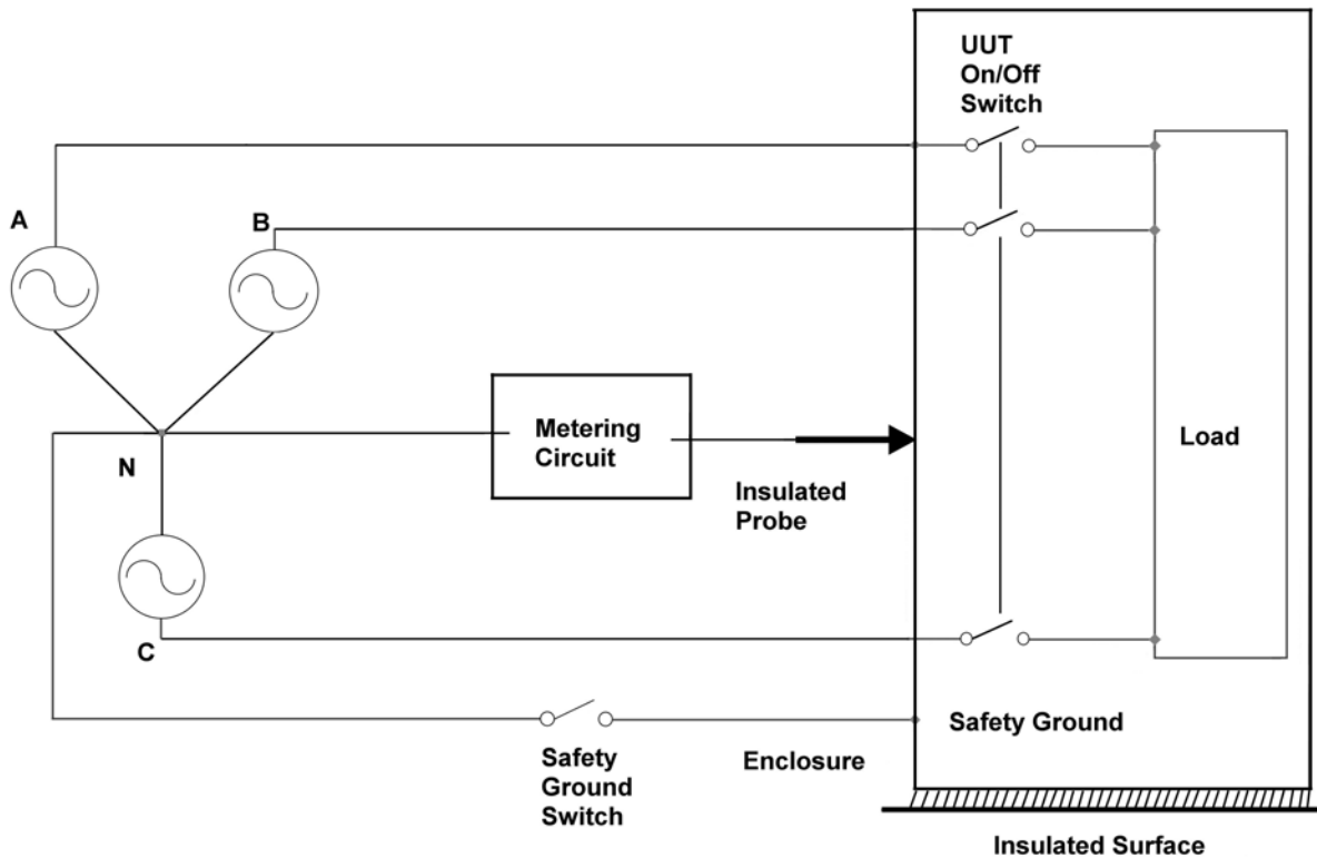
FIGURE 30. Three-phase simulated human body leakage current test setup for user equipment.
